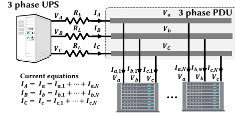
Figure 27: Three-phase distribution with three-phase server/server racks.
