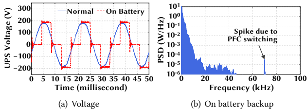
Figure 23: (a) Voltage reading at the PDU with the UPS running in normal mode and in battery-backup mode. (b) The PSD spike from server power supply unit is still visible with the non-sinusoidal voltage during the battery-backup mode.
