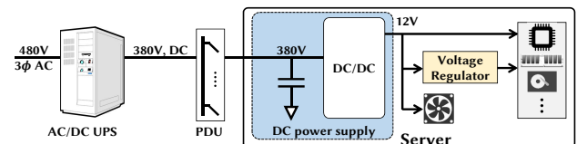
Figure 25: DC power distribution with DC server power supply unit that has no PFC circuit.
