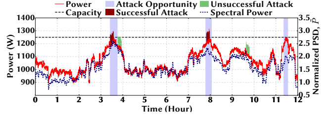
Figure 13: Illustration of power attack.
