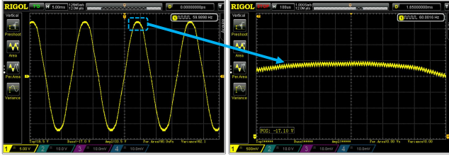
Figure 7: High-frequency voltage ripples at the PDU caused by switching in the server power supply unit.
