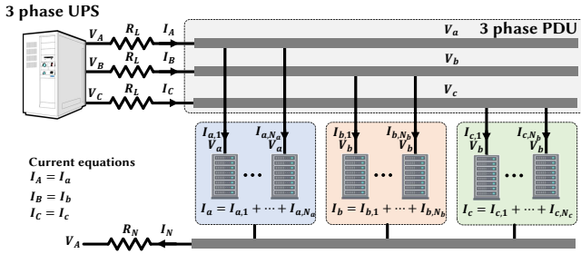
Figure 26: Three-phase distribution with single-phase, 120V server/server racks.
