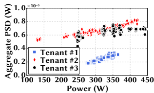
Figure 22: Power vs. PSD plot of different server groups.
