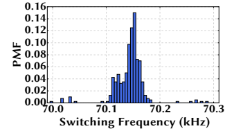
Figure 28: PMF shows the PFC switching frequency only fluctuates slightly.
