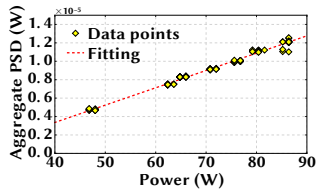
Figure 21: Server power vs. PSD aggregated within the bandwidth of 63 ~ 64kHz for the 350W PSU.
